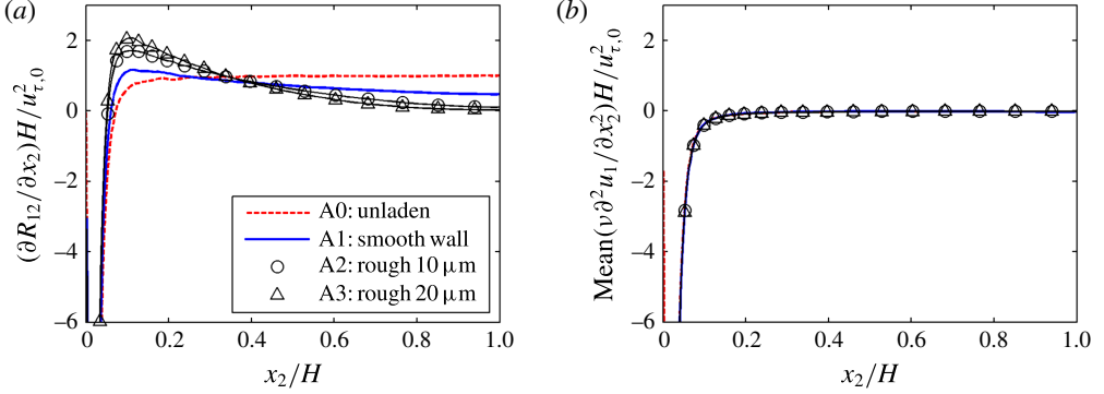
FIGURE 6. (Colour online) Differentiated Reynolds shear stress (a) and the mean of the viscous term in the streamwise component of the gas momentum equation (b), normalized with \rho u_{\tau,0}^2/H . Laden simulations A1 (solid, no markers), A2 (solid, circles) and A3 (solid, triangles).
