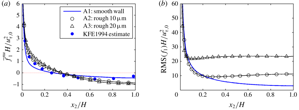
FIGURE 5. (Colour online) Non-uniform part (a) and RMS (b) of the particle drag force in the streamwise component of the gas momentum equation, \bar{f}_1^{\text{nu}} and \text{RMS}(f_1) , normalized with \rho u_{\tau,0}^2/H . Laden simulations A1 (solid, no markers), A2 (solid, circles) and A3 (solid, triangles). In (a) an estimate based on experimental results (KFE1994) is also shown, as described in the text.
